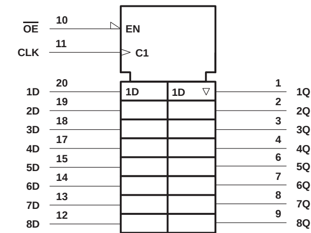
logic symbol†
